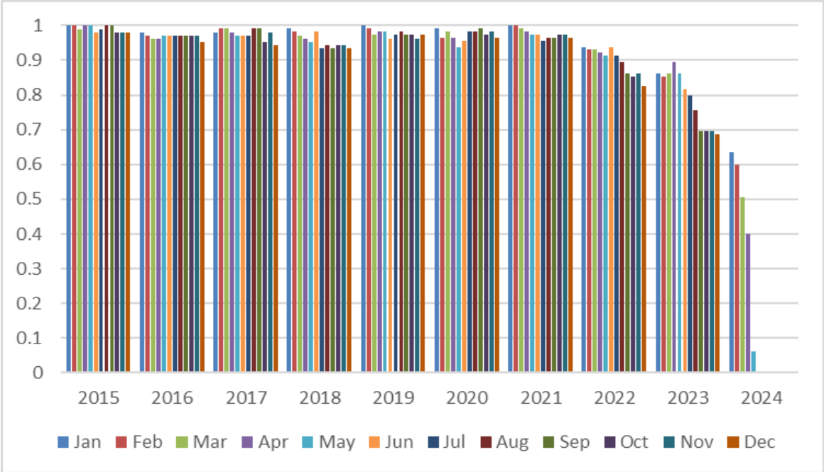
Fig.1 Percentage of Monthly Ward Discharges Submission from January 2015 May 2024
